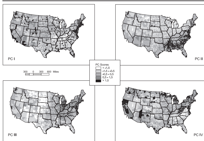
FIGURE 6. Principal Component (PC) Scores for 1990
